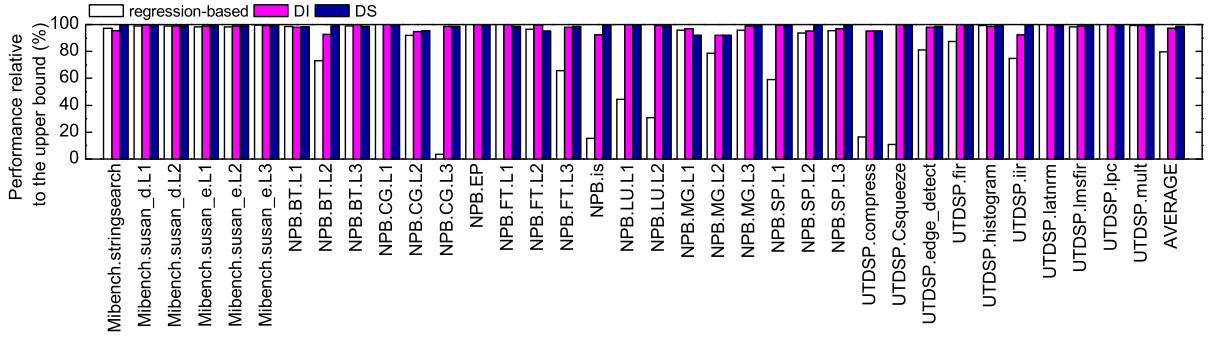
Figure 12. Performance relative to the upper bound on the Intel platform. Our machine learning based predictors have the closest performance to the upper bound (96% and 97% compared with 80%).
