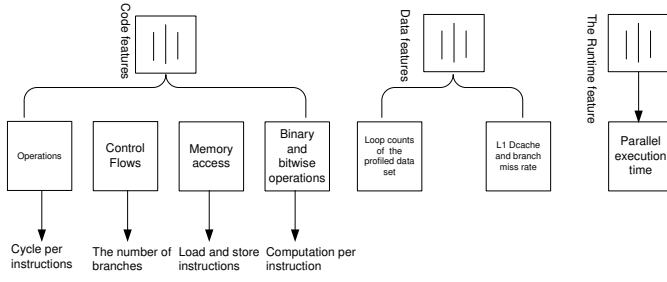
Figure 8. Feature data is processed into feature groups.
