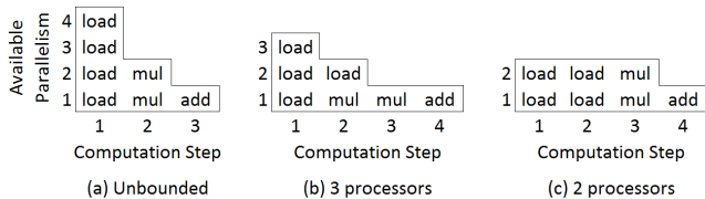
Figure 5. Parallelism profiles for the dot-product code.
