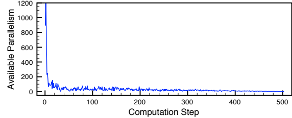
Figure 21. Parallelism profile for ordered agglomerative clustering
