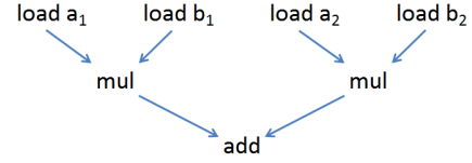
Figure 4. The computation DAG of (a_1 * b_1) + (a_2 * b_2) .
