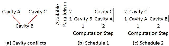
Figure 6. Parallelism graph with multiple resulting schedules.
