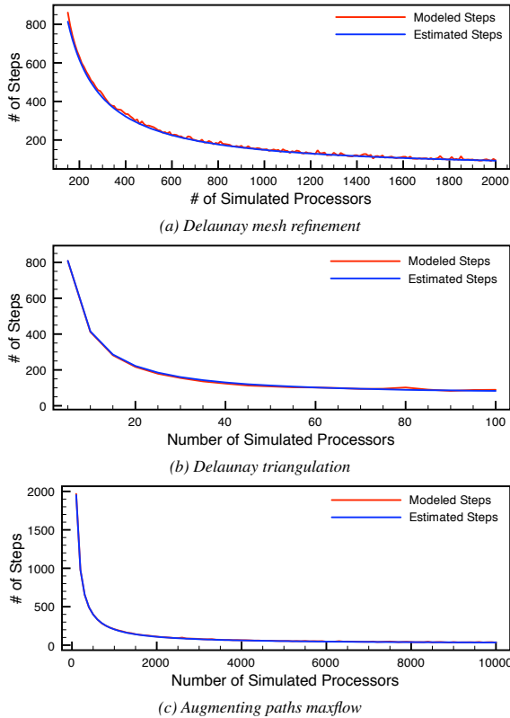
Figure 22. Constrained parallelism: measured vs. estimated.
