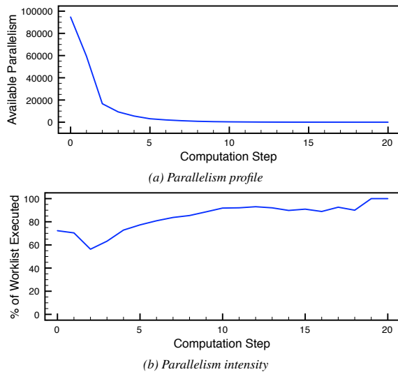
Figure 13. Parallelism metrics for augmenting paths maxflow.
