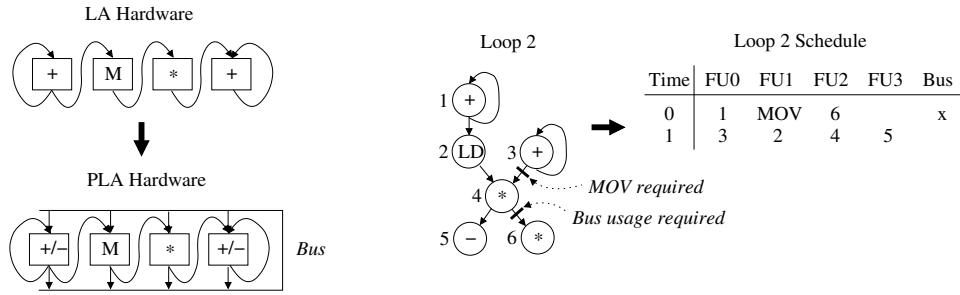
Figure 7: PLA generalization and scheduling example.
