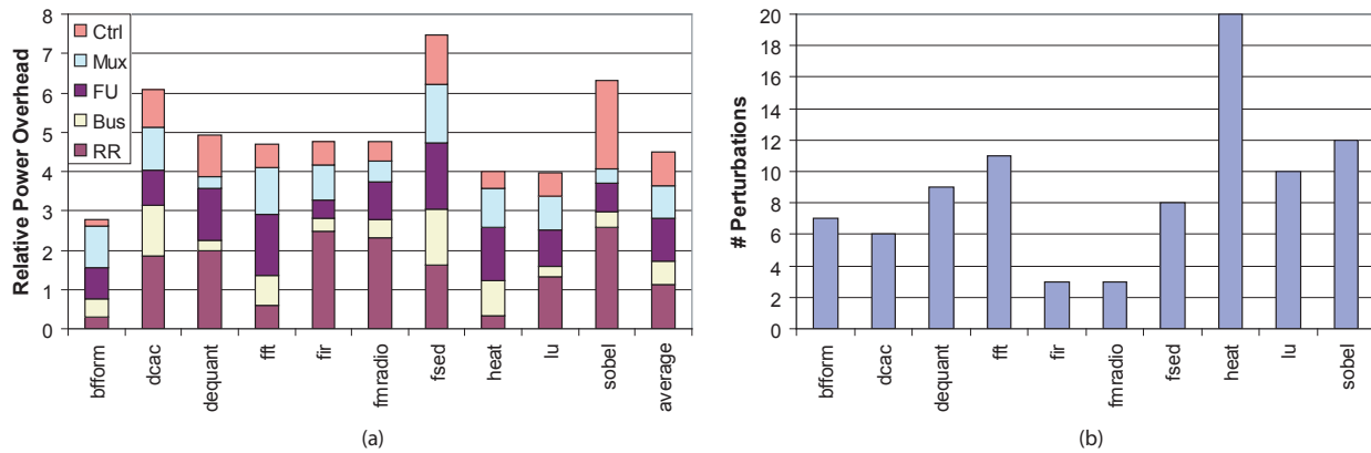
Figure 11: (a) Power consumption breakdown of PLA generalizations. (b) Number of perturbations achieved without loss of performance.
