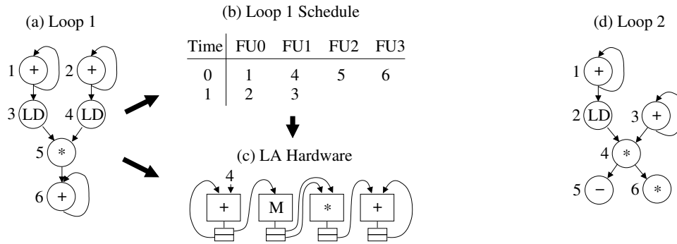
Figure 5: LA scheduling and synthesis example.
