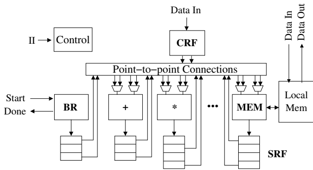
Figure 4: Template for single-function loop accelerator.
