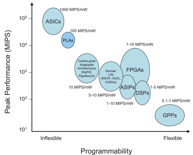
Figure 1: Comparison of peak performance, power efficiency, and programmability of different architecture design styles.
