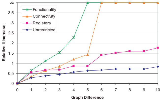
Figure 6: Average performance degradation resulting from LA datapath restrictions.
