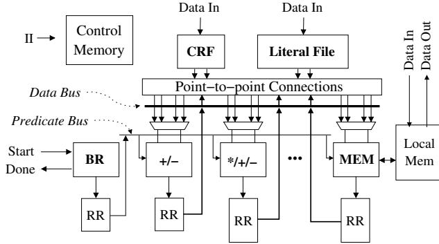
Figure 8: Template for programmable loop accelerator.
