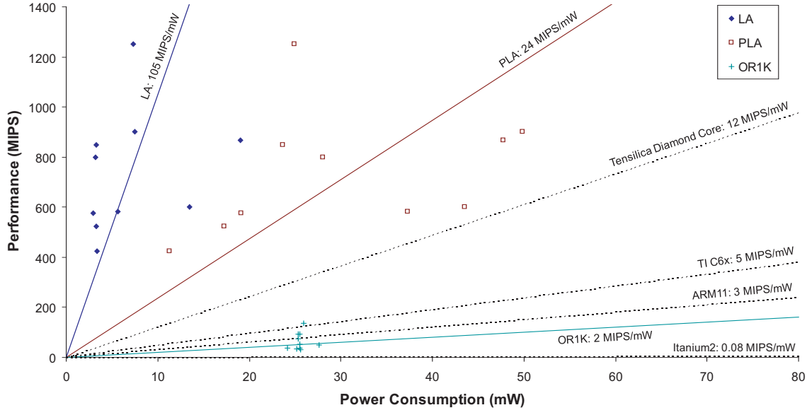
Figure 10: Performance/power of loop accelerators and OR-1200.
