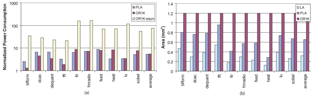
Figure 9: (a) Power consumption of PLA and OR-1200 relative to single-function LA. (b) Area of loop accelerators and OR-1200.
