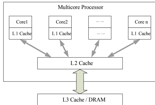
Fig. 5 Multicore Architecture
