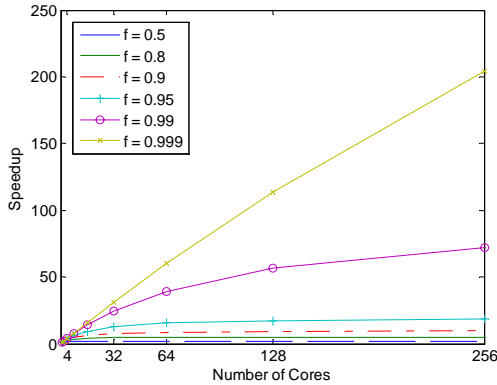
Fig. 1 Fixed-size Speedup of a Multicore Architecture
