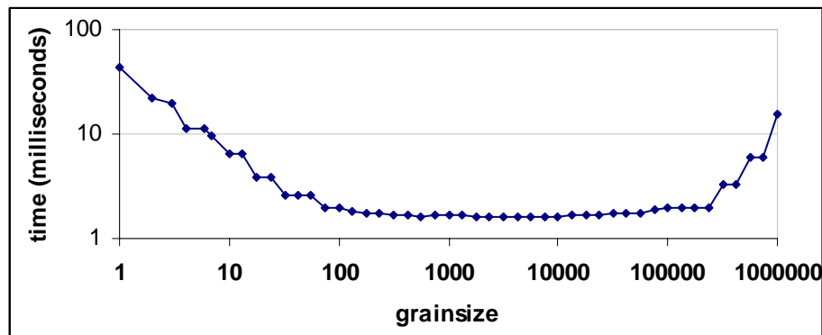
Figure 3: Wallclock Time Versus Grainsize
